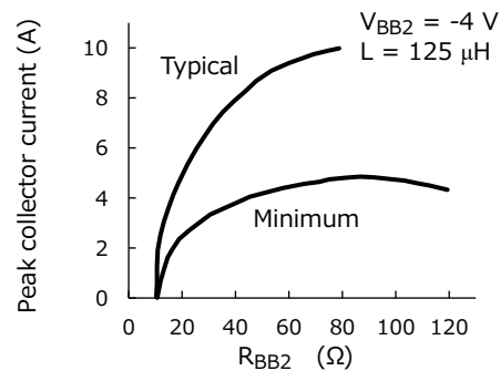
(c) Dependence on the base voltage V_{BB2}
