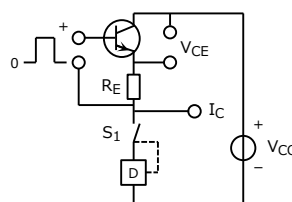
D : Detection and protection circuit S1: Switch controlled by a signal from D
