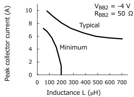
(b) Dependence on the base resistor R_{BB2}
