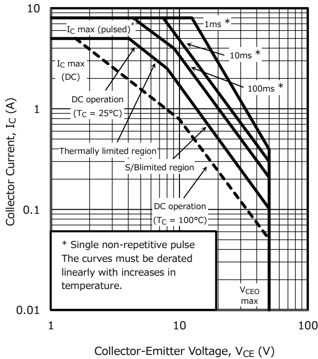
Figure 1.16 SOA for Transistor A and an example of SOA derated for T_C = 100^\circ\text{C}
