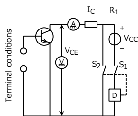
D : S/B detection and protection circuit S1, S2 : Switches controlled by signals from D
