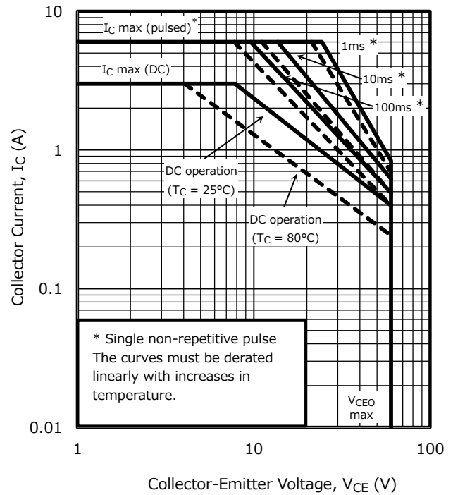
Figure 1.17 SOA for Transistor B and an example of SOA derated for T_C = 80^\circ\text{C}
