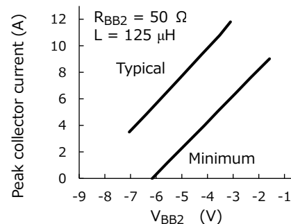
Figure 1.19 Examples of reverse-bias SOAs
